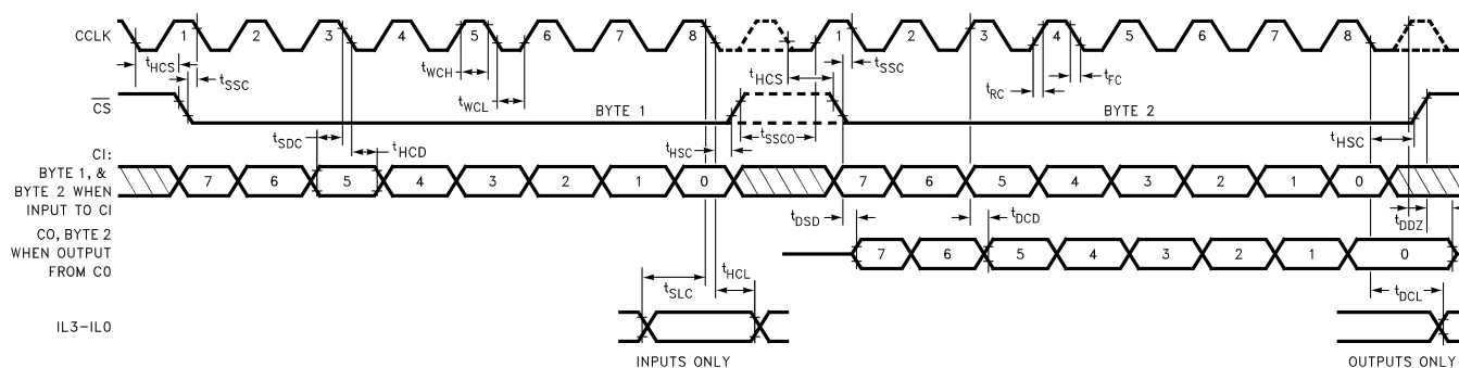
Figure 4. Control Port Timing
