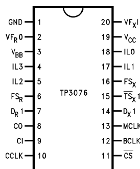
Figure 1. See Package PDIP (NHF)
